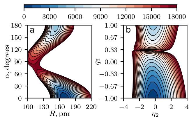
Figure 4. Two-dimensional cuts of the HCN/HNC potential energy surface. (a) Cut along the Jacobi coordinates R and \alpha_{\text{R-CN}} . (b) Cut along the optimized normalizing-flow coordinates. The optimization was performed for a basis set truncated at P_{\max} = 16 (285 basis functions), with the loss function defined as the sum of the 100 lowest vibrational state energies. An effective decoupling of the surface in the normalizing-flow coordinates is patent.
